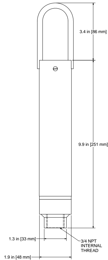
CT-201GC-3/4 PROBE
