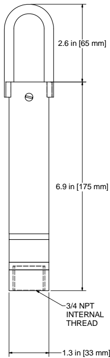
CT-200GC PROBE
